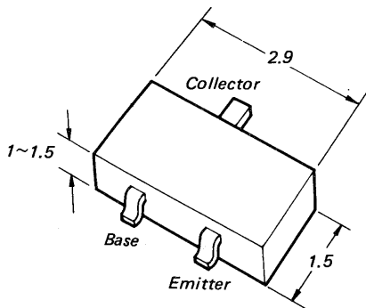
Transistor
