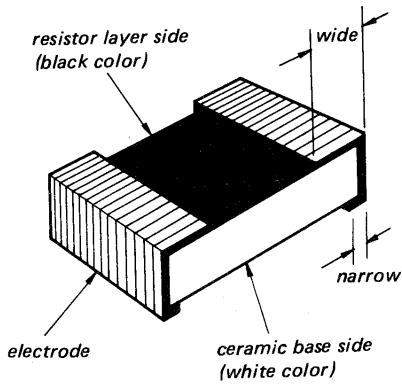
Resistor
