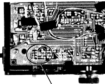
LEVEL/BATT meter
