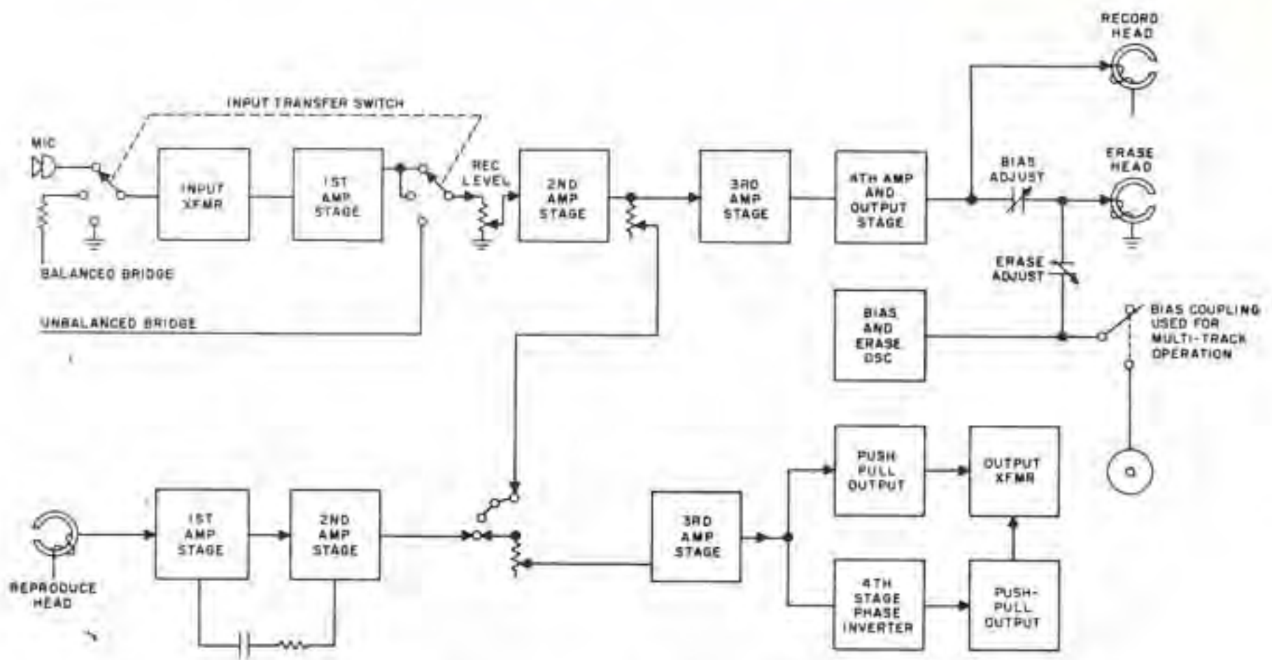
SYSTEM BLOCK DIAGRAM
