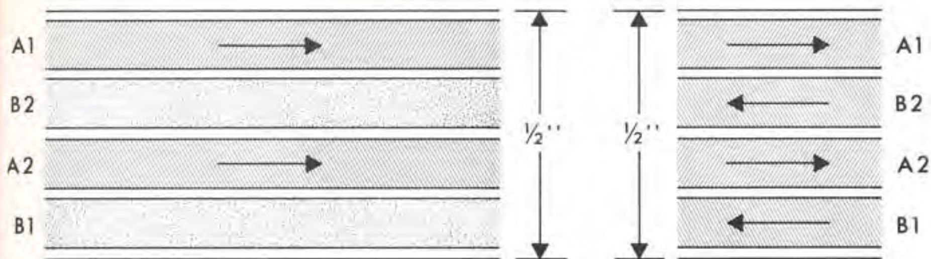
TRACK CONFIGURATION MODEL 300-2M
