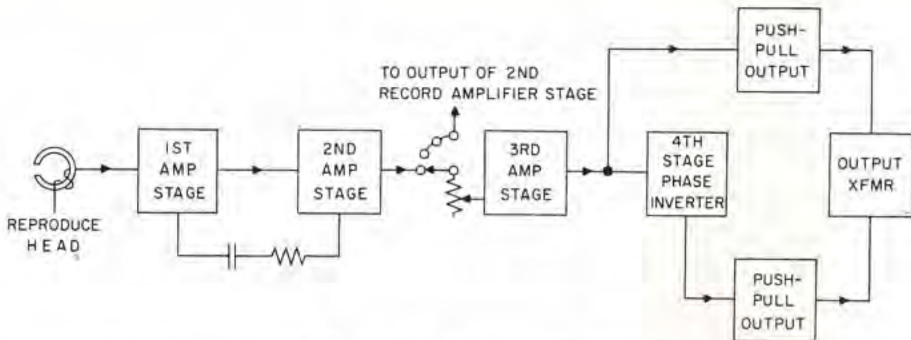
BLOCK DIAGRAM REPRODUCE CIRCUIT
