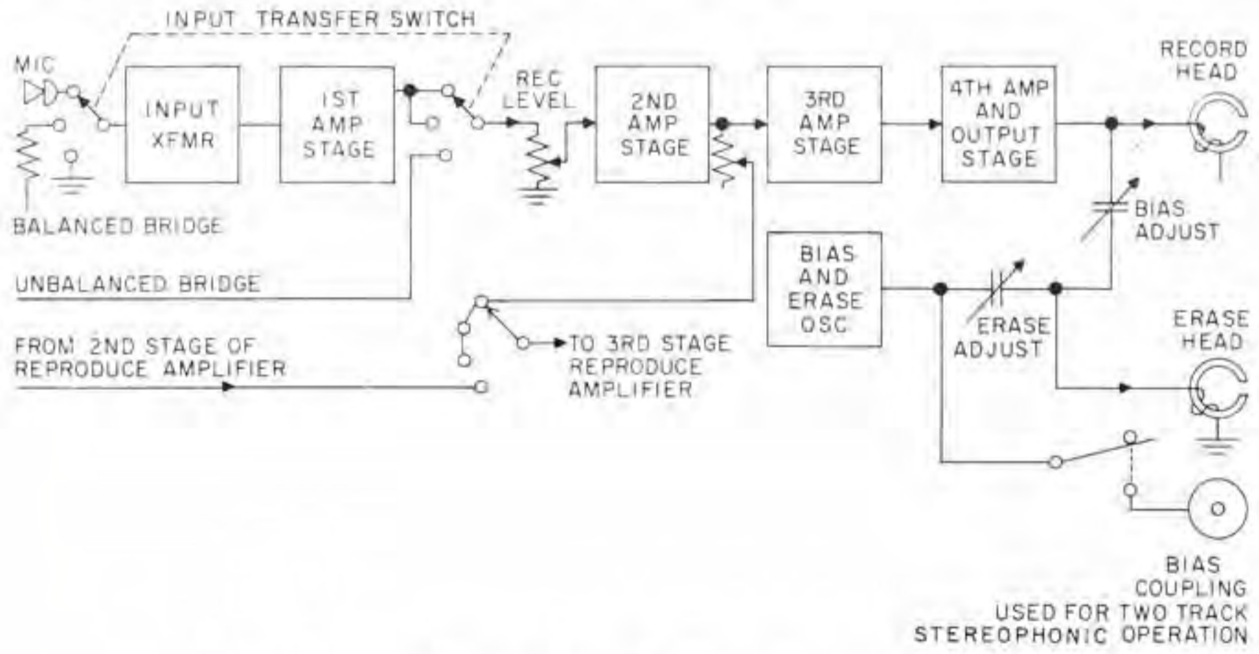
BLOCK DIAGRAM RECORD CIRCUIT
