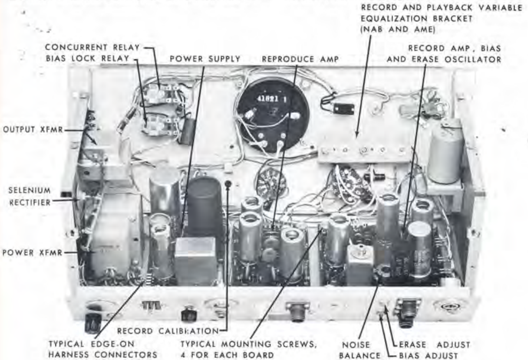
LOCATION OF ELECTRONIC SUBASSEMBLIES
