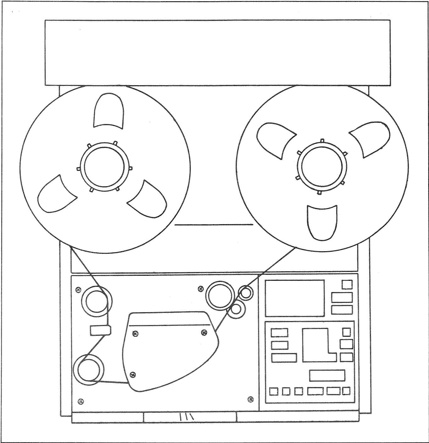
Figure 4-10. Tape Path
