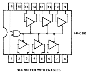
HEX BUFFER WITH ENABLES
