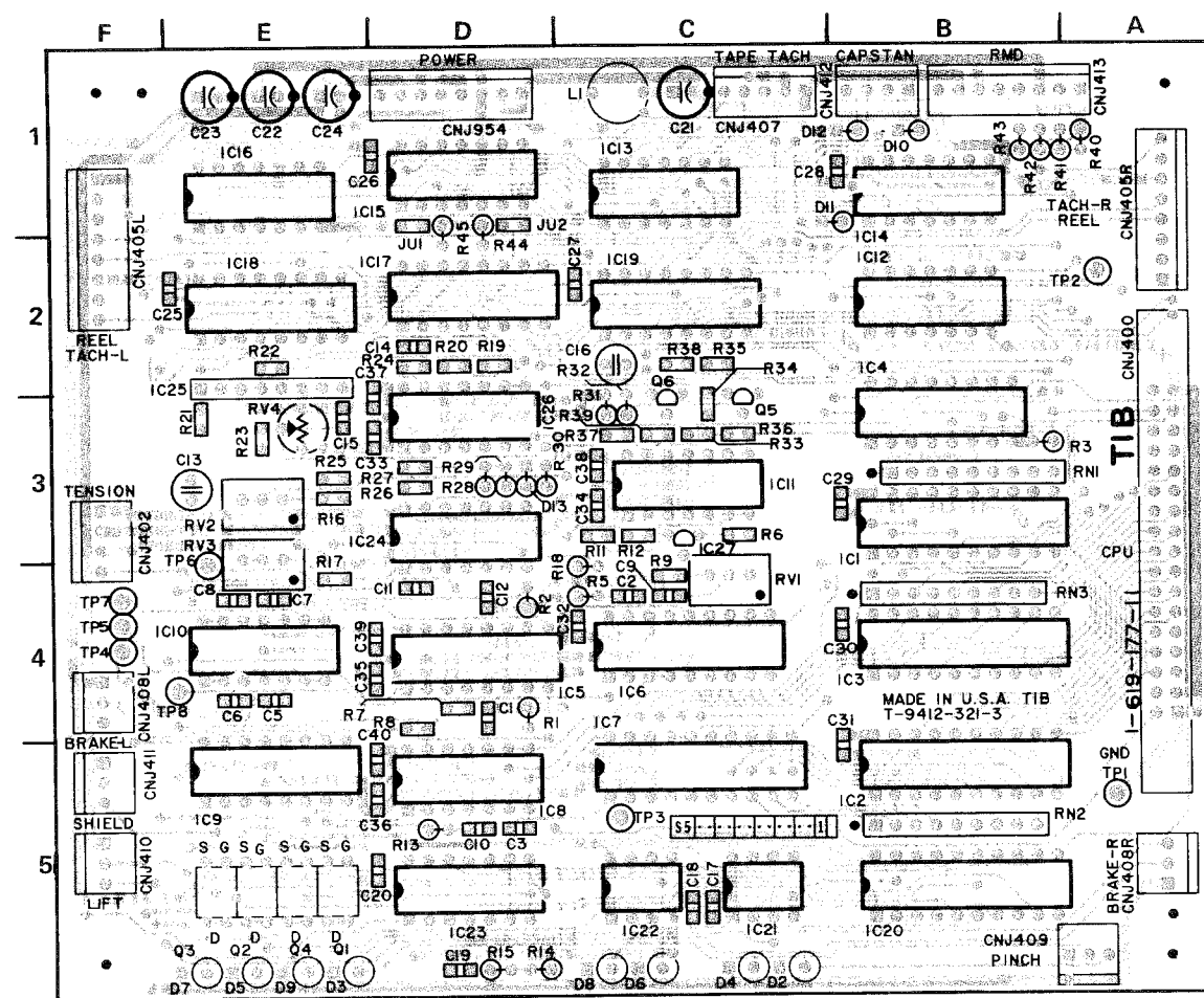
TIB BOARD (1-619-177-11) Component Side
