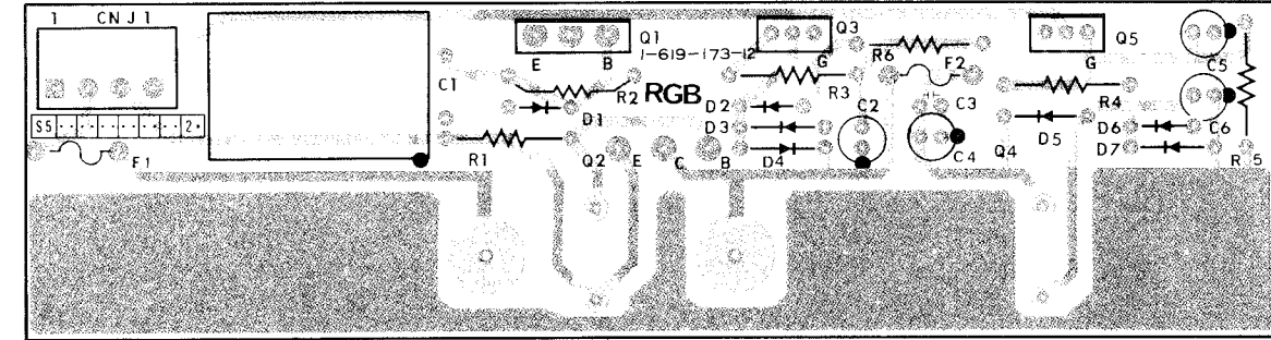
3 SOLDER SIDE PATTERN 1-619-173-12
