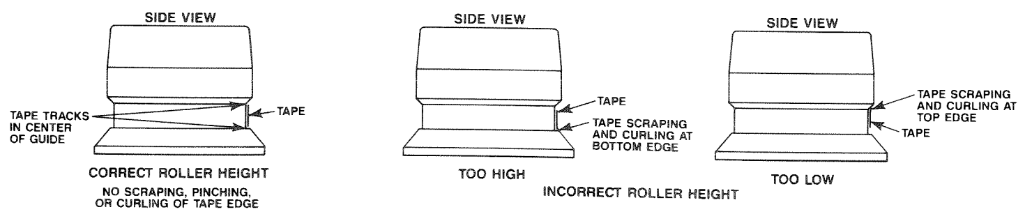
Figure 6-24. Tape Path Over the Roller Guides
