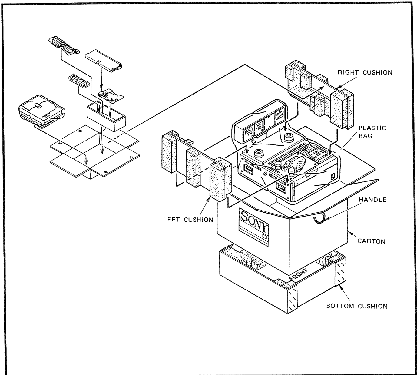
Figure 2-1. APR-5000 Packaging
