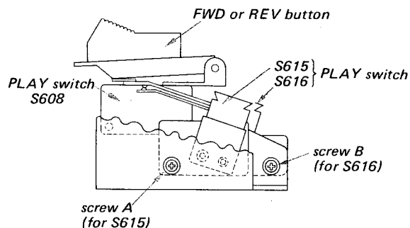
Fig. 3-23. PLAY switch (S615, 616) position adjustment
