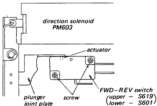
Fig. 3-18. FWD/REV switch (S601, 619) position adjustment
