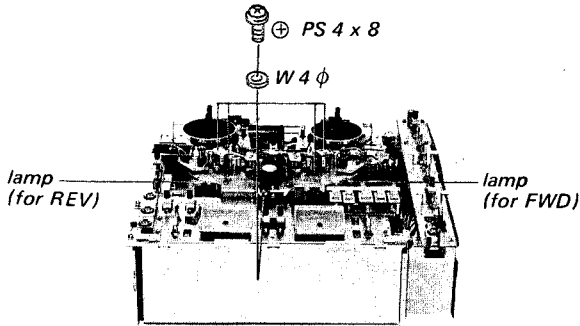
Fig. 2-2. Head deck removal
